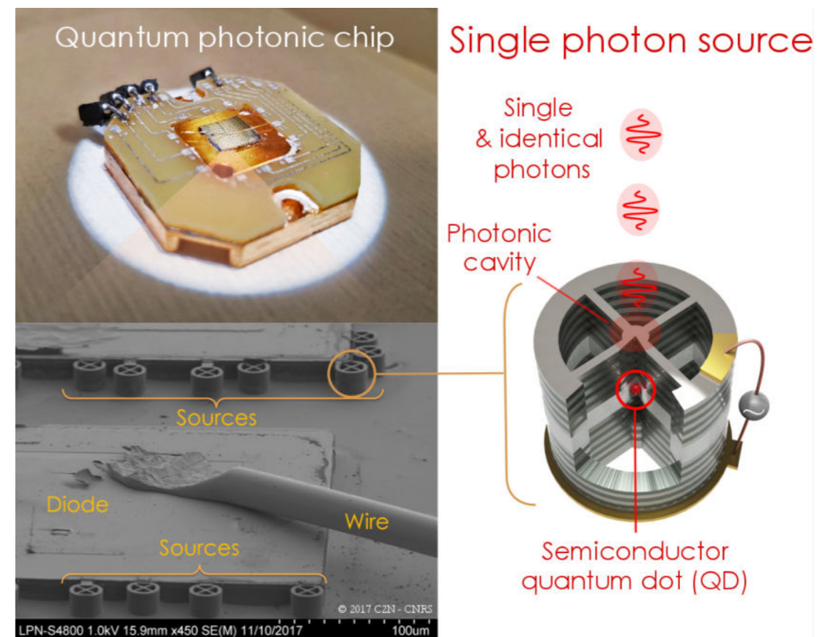
QD-based single-photon source (courtesy of Quandela)
